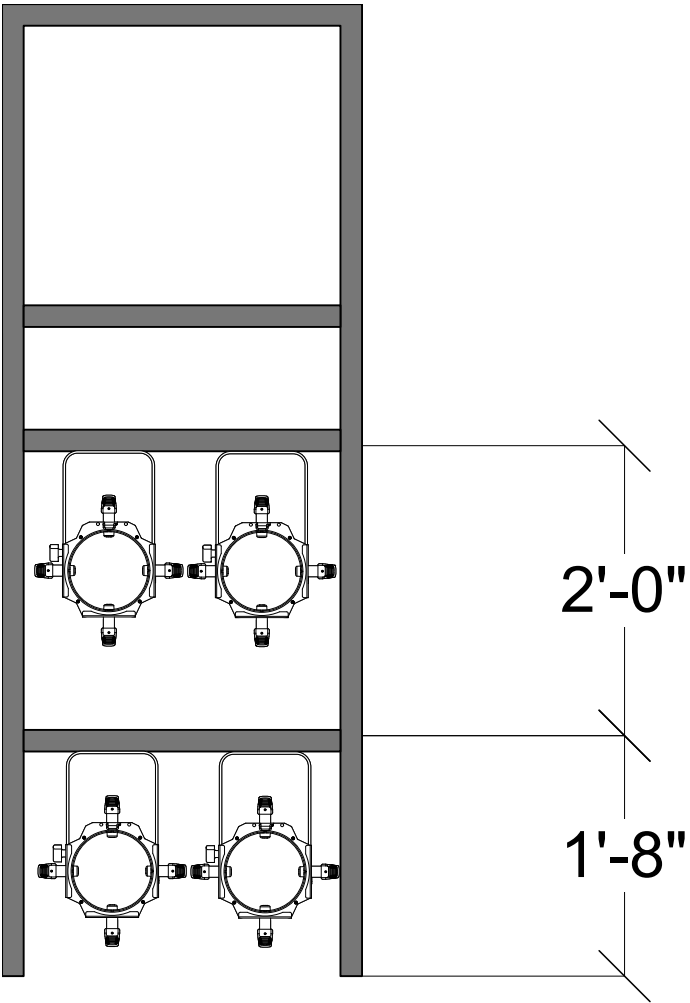
Front Elevation
